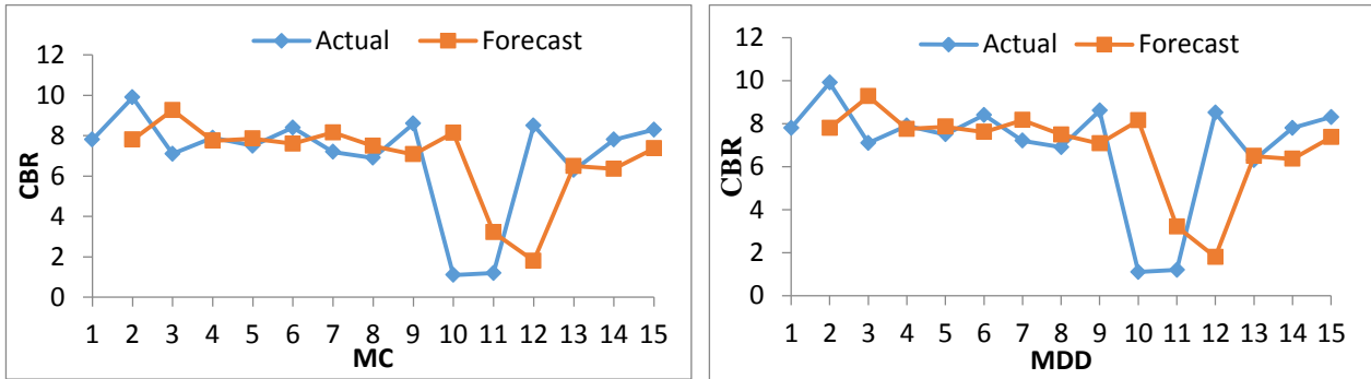
Figure 9: Comparison between actual values and forecast values of CBR for MC and MDD
