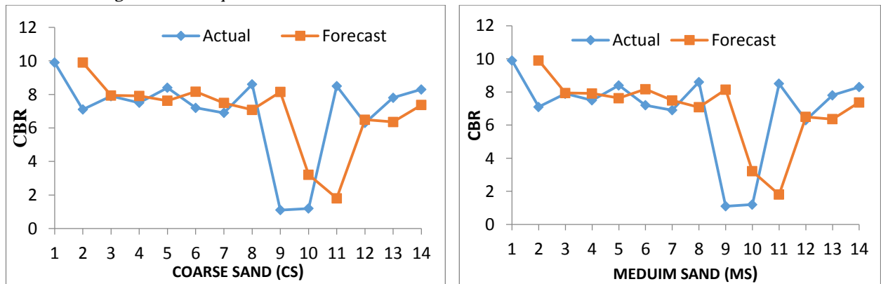
Figures 11: Comparison between Actual values and forecast values CBR CS and MS
