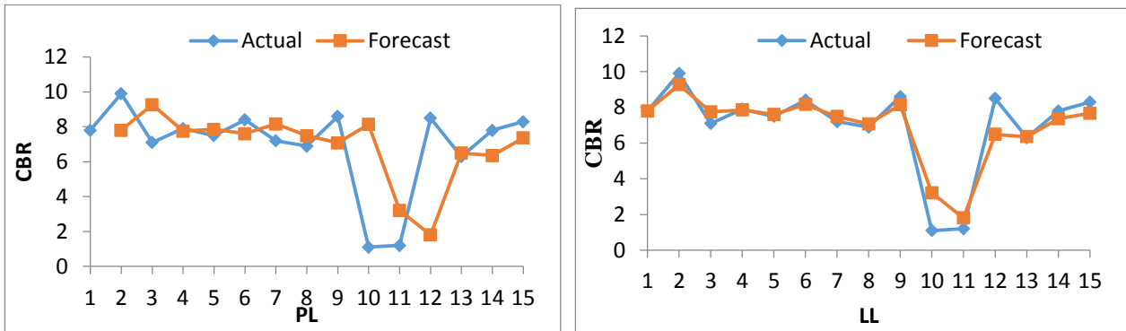
Figure 10: Comparison between actual values and forecast values of CBR for PL and LL
