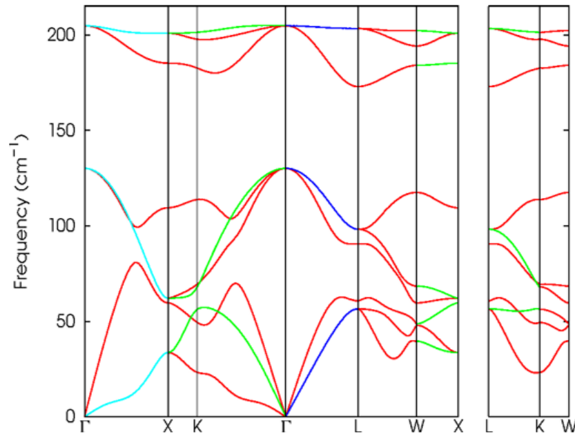
Fig. 4. Calculated phonon frequency versus wave vector coordinate for NaCrSb
