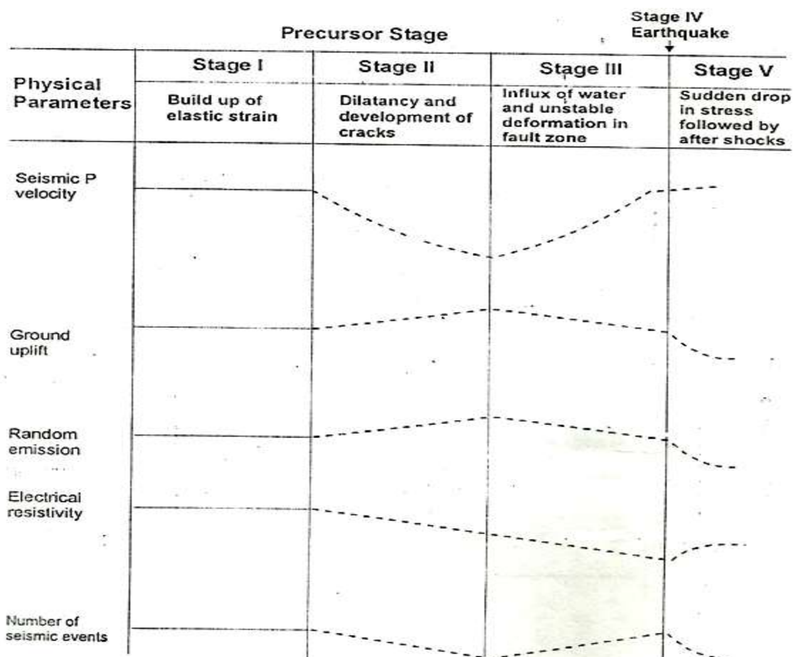
FIGURE 1: PHYSICAL CLUES FOR EARTHQUAKE PREDICTION (Source: Culled from G. A. Eiby 1982)
