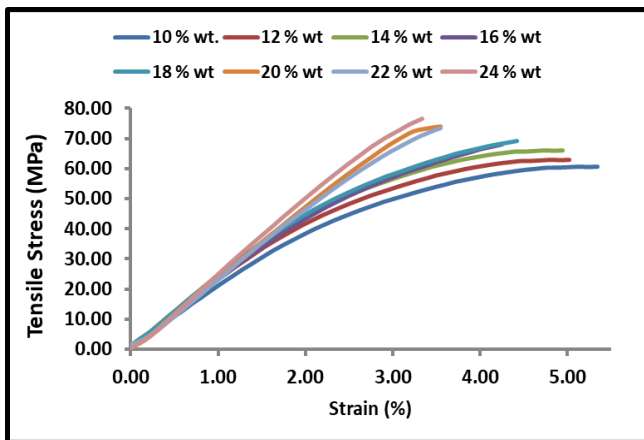
Figure 2: Stress-strain curves of polyester reinforced bamboo composite
