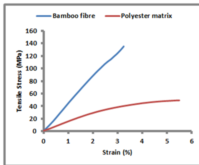
Figure 1: Stress-strain curves of polyester and bamboo
