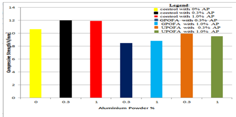
Figure 4.3: Compressive Strength and Aluminum Content after 28 days
