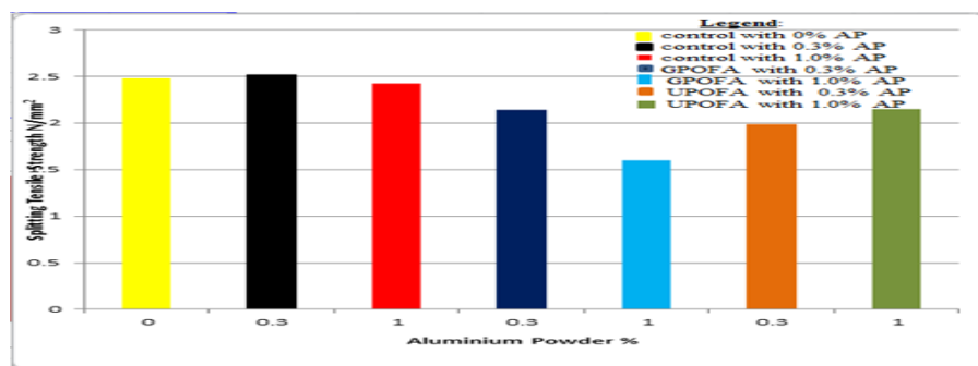
Figure 4.4: Tensile Spitting Strength VS Aluminum Content after 28 days
