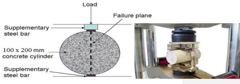
Figure 3.3: Splitting Tensile Specimen and Test Machine
