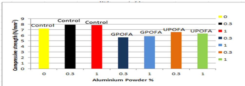
Figure 4.1: Compressive Strength and Aluminium Content after 7 days
