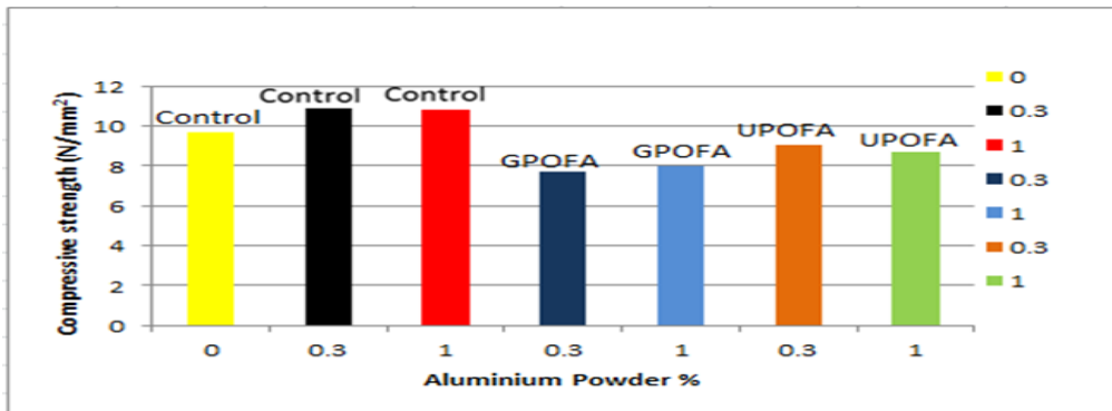
Figure 4.2: Compressive Strength VS Aluminium Content after 14 days
